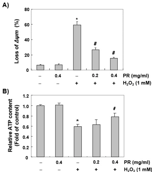
Fig. 6. Prevention of H 2 O 2 -induced mitochondrial dysfunction by PR in Chang liver cells.
