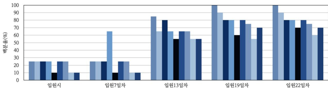
Fig. 2. The change of the temperature sensation.
